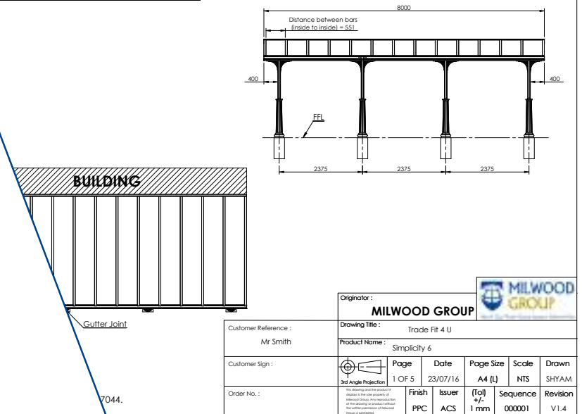
FRONT VIEW & ROOF TOP VIEW WITH BUILDING
