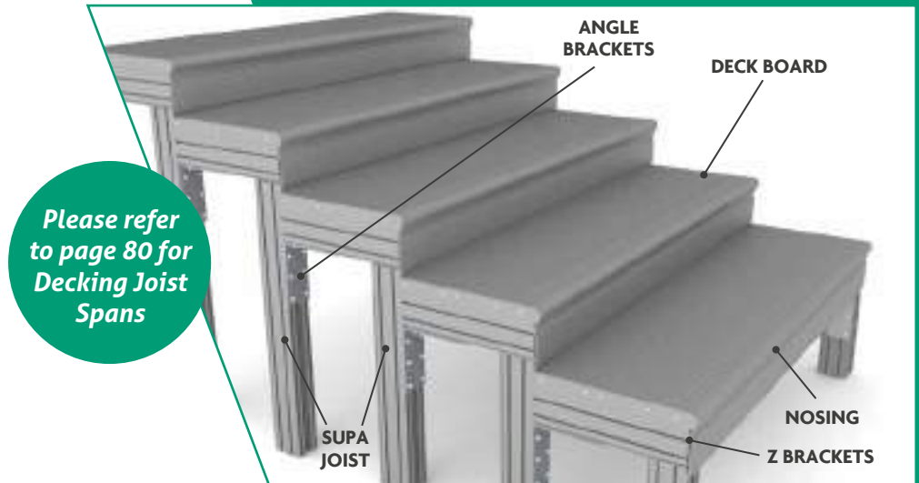
Stairs & Nosing
